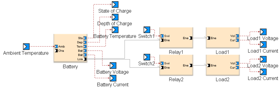
Fig. 7. Battery and DC loads configuration FACT model
