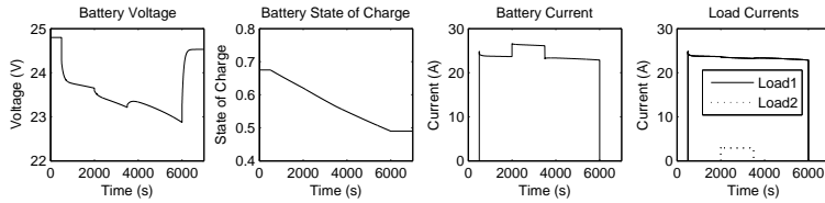
Fig. 8. Simulation results
