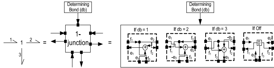
Fig. 5. Block Diagram expansion of a hybrid junction.
