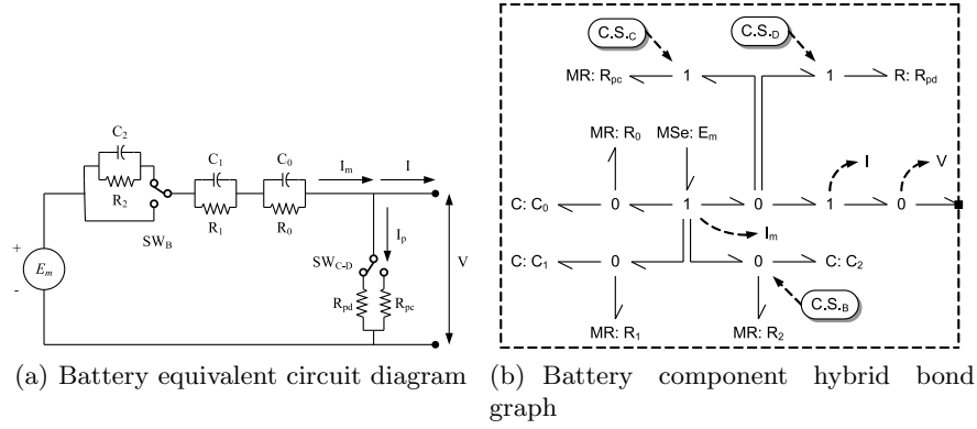
Fig. 6. Hybrid nonlinear battery model
