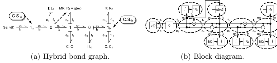
Fig. 4. Example system with junction 1_a off.
