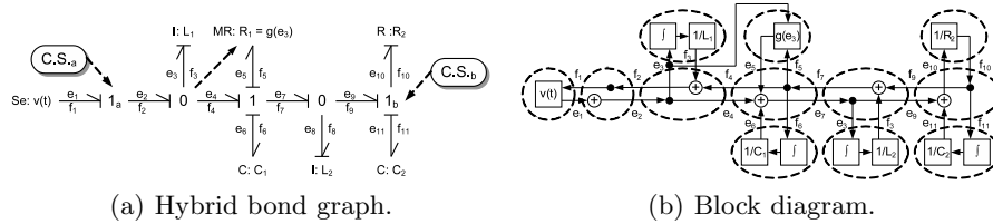
Fig. 3. Example system with both switches on.
