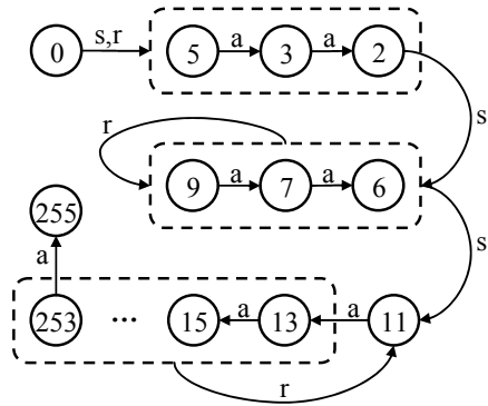
Fig. 4. The state machine of the reliable broadcast policy
