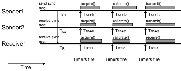
Figure 2: The synchronization schedule that aligns the start of the transmission and reception at multiple nodes.
