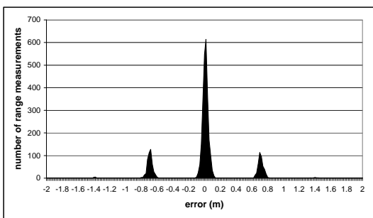
Figure 9: Error distribution of the filtered ranges.
