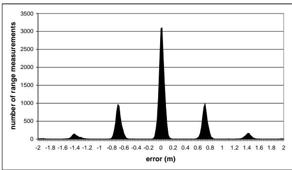
Figure 8: Error distribution of all the ranges.
